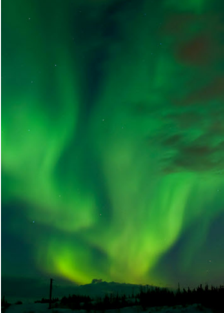
The aurora borealis in Canada - the result of particles from the sun colliding with oxygen and nitrogen atoms in the Earth's atmosphere. Image: D. Dyet, www.rgbstock.com
